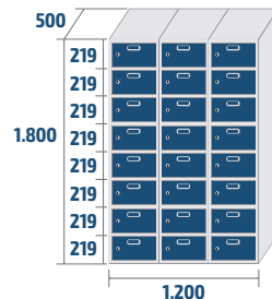
ECOZ-40/3 COD: 84823 82,7kg · 1,08m 3
